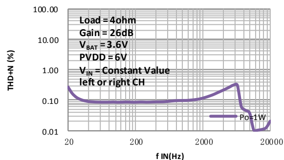
f_{IN} vs THD+N
