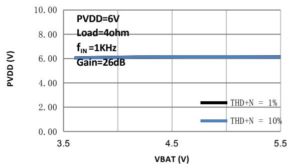
V BAT vs P VDD
